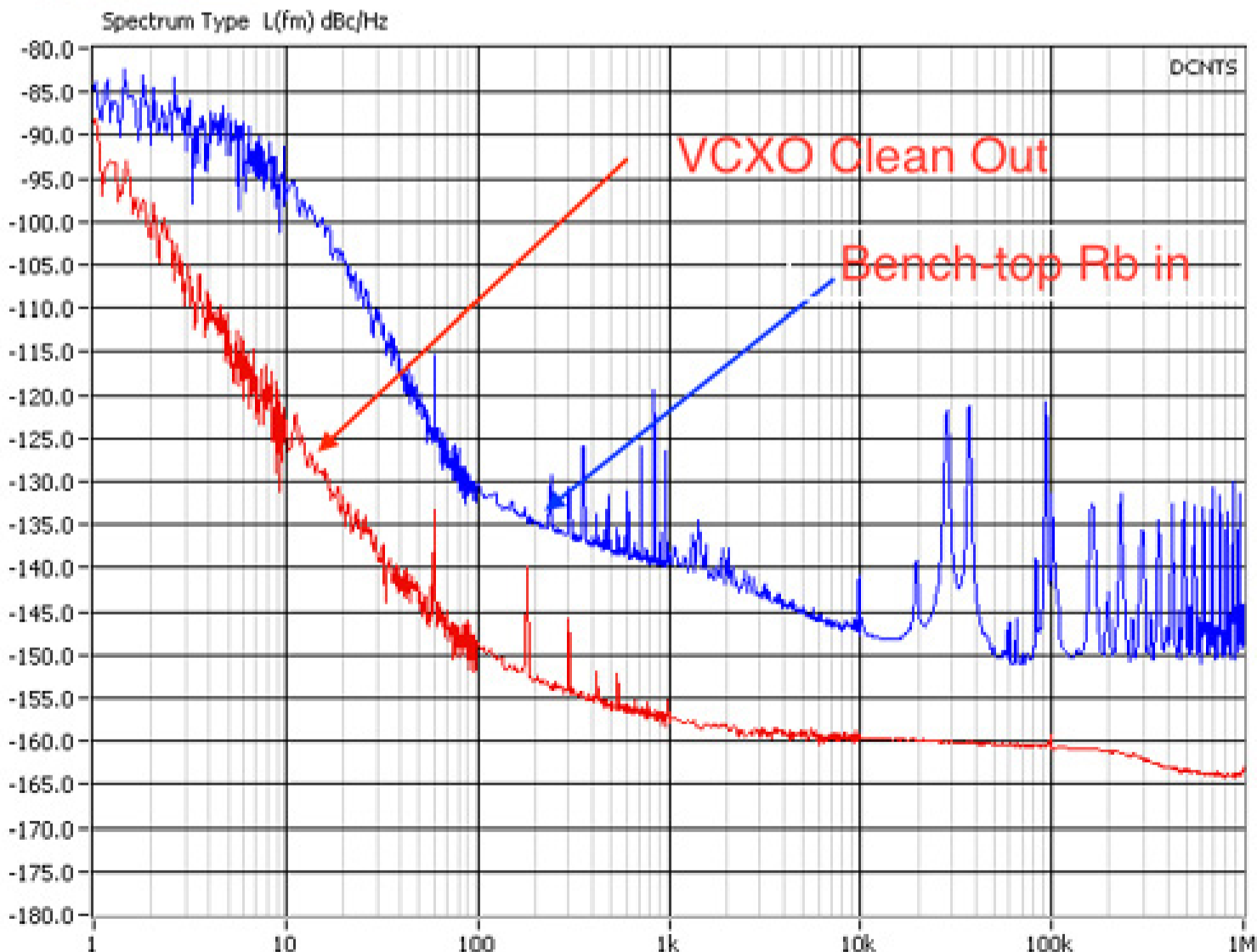
Phase Noise Plot
